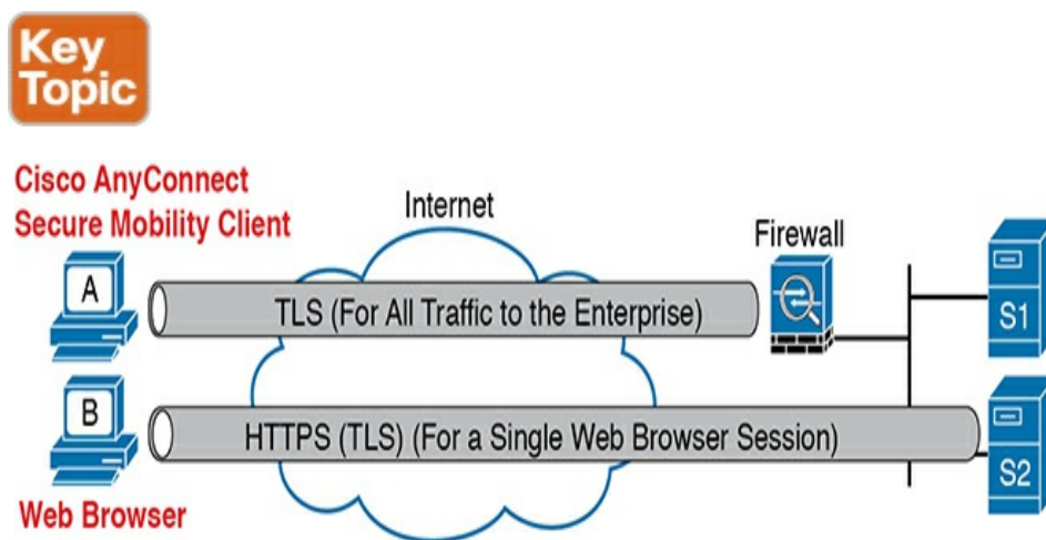
Figure 14-23 Remote Access VPN Options (TLS)
