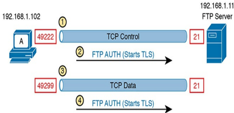
Figure 12-20 FTPS Explicit Mode Control and Data Connection Establishment
