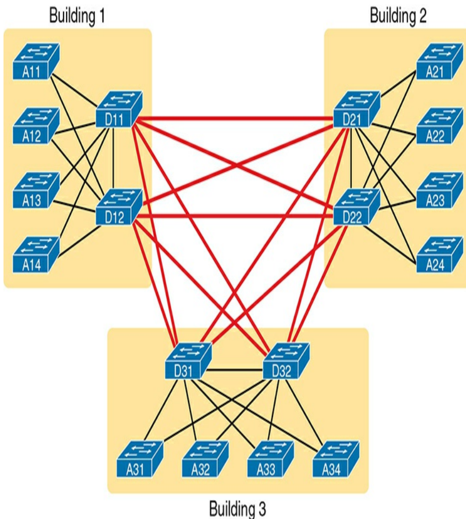
Figure 13-4 Two-Tier Building Design, No Core, Three Buildings
